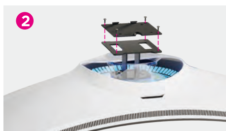
Attach the VESA Plate (not included)
